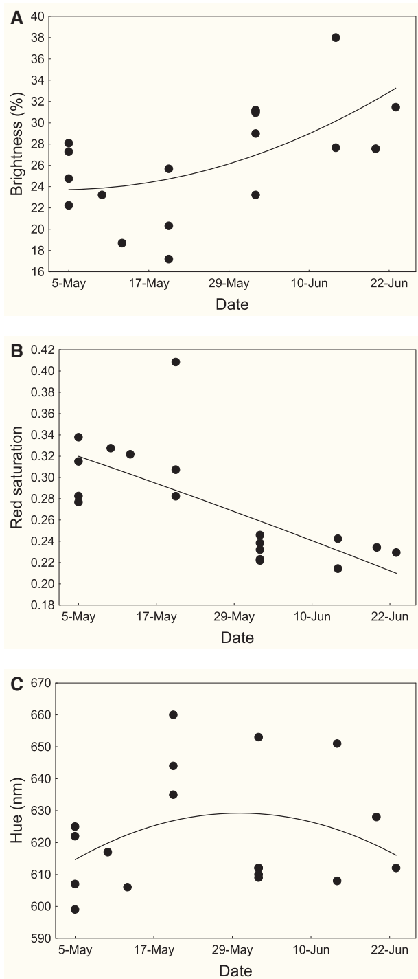
Figure 2. Mean (A) brightness, (B) red saturation, and (C) hue in 18 adult female spiny-footed lizards in the Madrid population during the 2011 reproductive season. Polynomial fit is represented as a continuous line for illustrative purposes.
